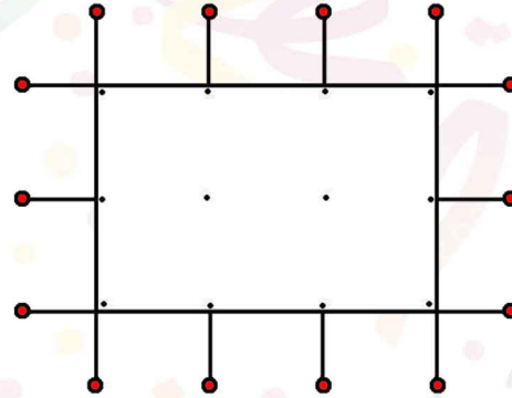
20x30 Stake & Pole Tent overhead layout of ANCHOR POINTS
